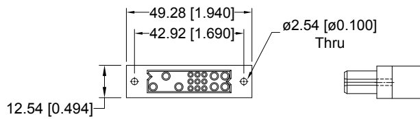
CONNECTOR DIMENSIONS
