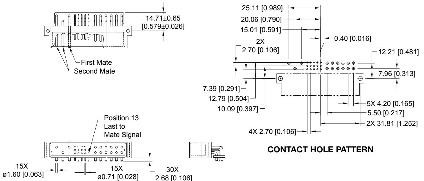
CONNECTOR DIMENSIONS
