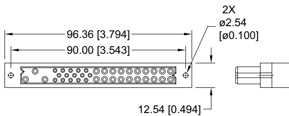
CONNECTOR DIMENSIONS
