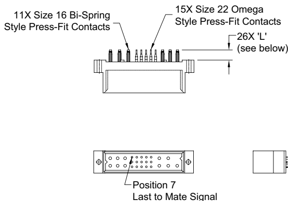
CONNECTOR DIMENSIONS
