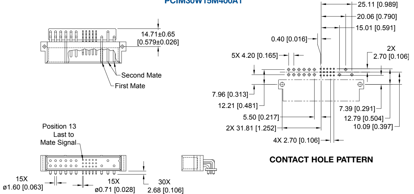
CONNECTOR DIMENSIONS
