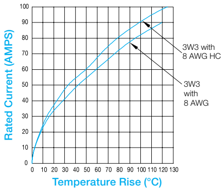
MCBX3W3 #8 Contacts
