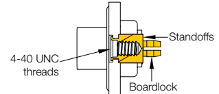
C8 Inside wall mount, 4-40 standoffs with boardlocks, for use with straight PCB termination types
