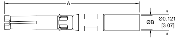
FEMALE CONTACT
