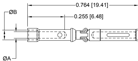
FEMALE CONTACT
