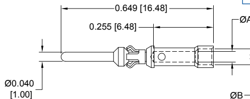
MALE CONTACT
