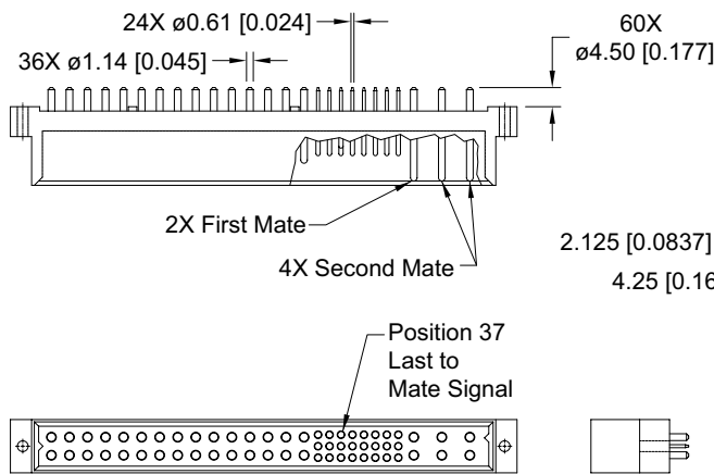
CONNECTOR DIMENSIONS
