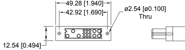
CONNECTOR DIMENSIONS
